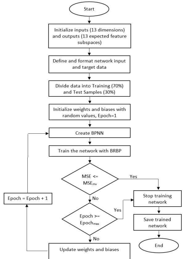
Fig. 2 Training process flowchart of the ANN for LDA/GSVD
