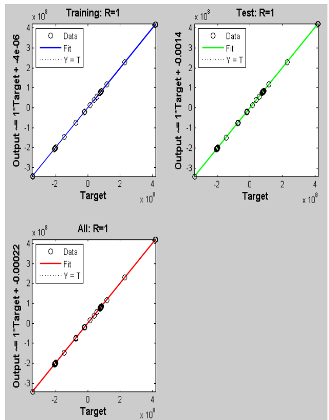
Fig. 8. BRBP's Regression Analysis
