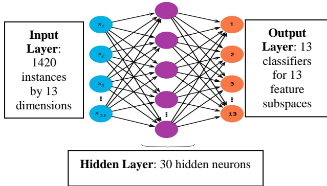
Fig. 3 Artificial Neural Network Architecture for the LDA/GSVD algorithm
